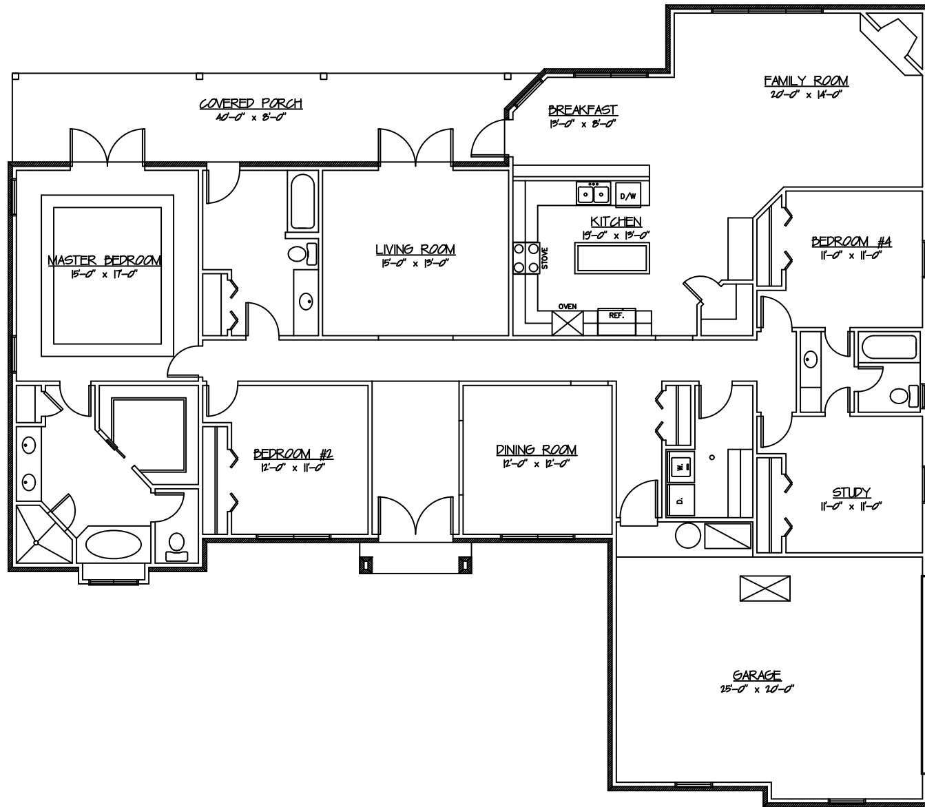
FLOOR PLAN
