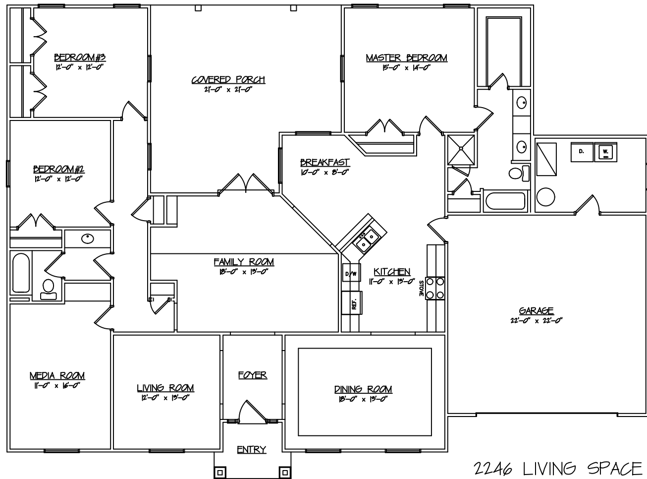
FLOOR PLAN
