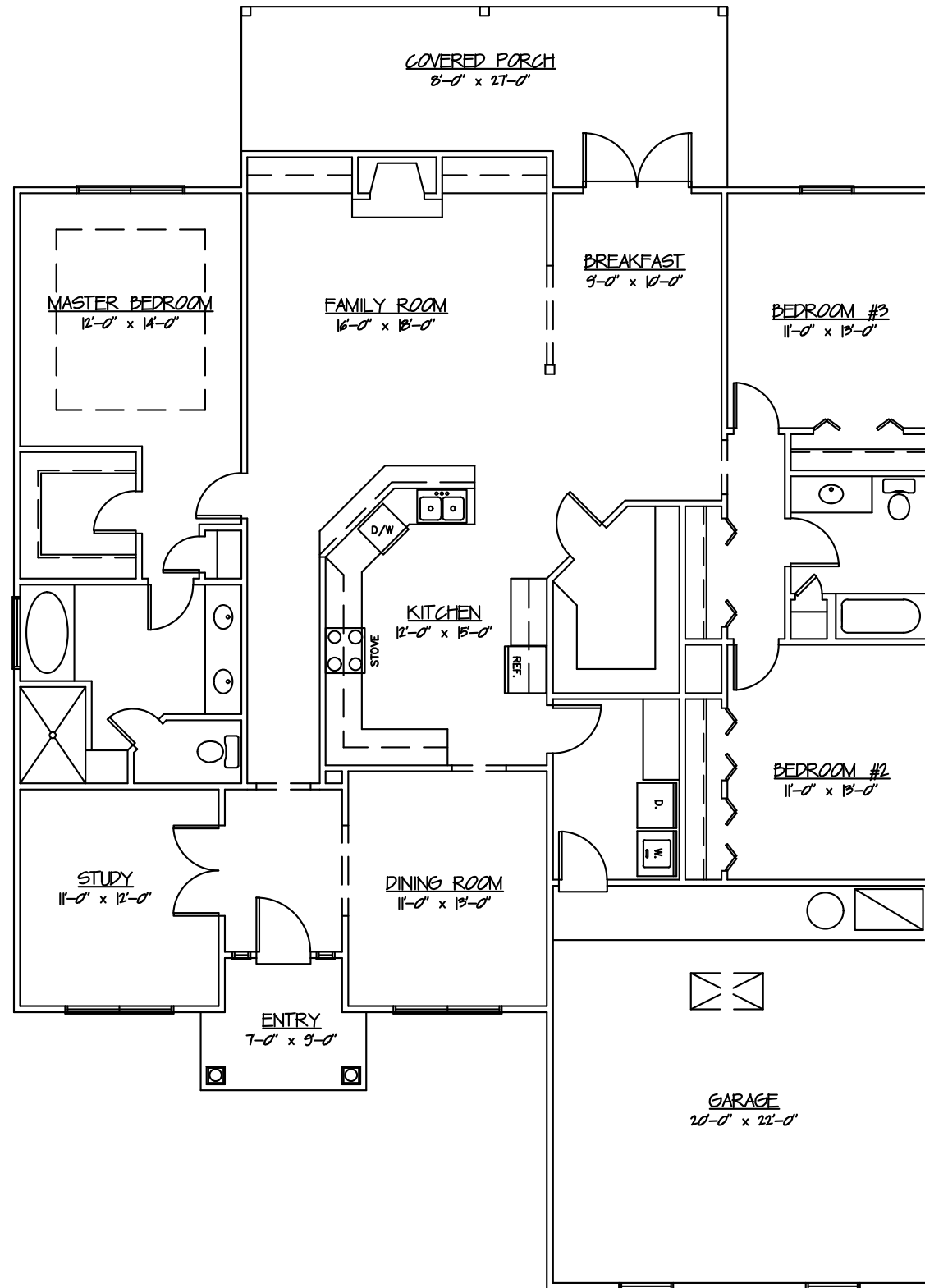
FLOOR PLAN
