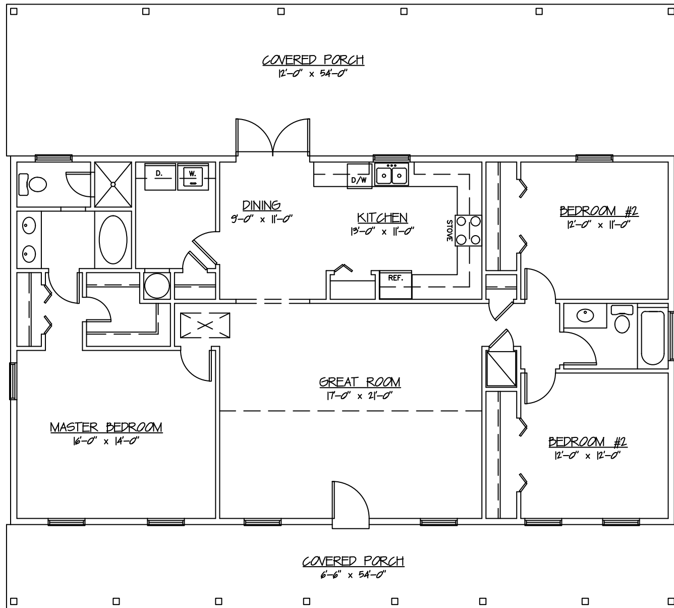
FLOOR PLAN
