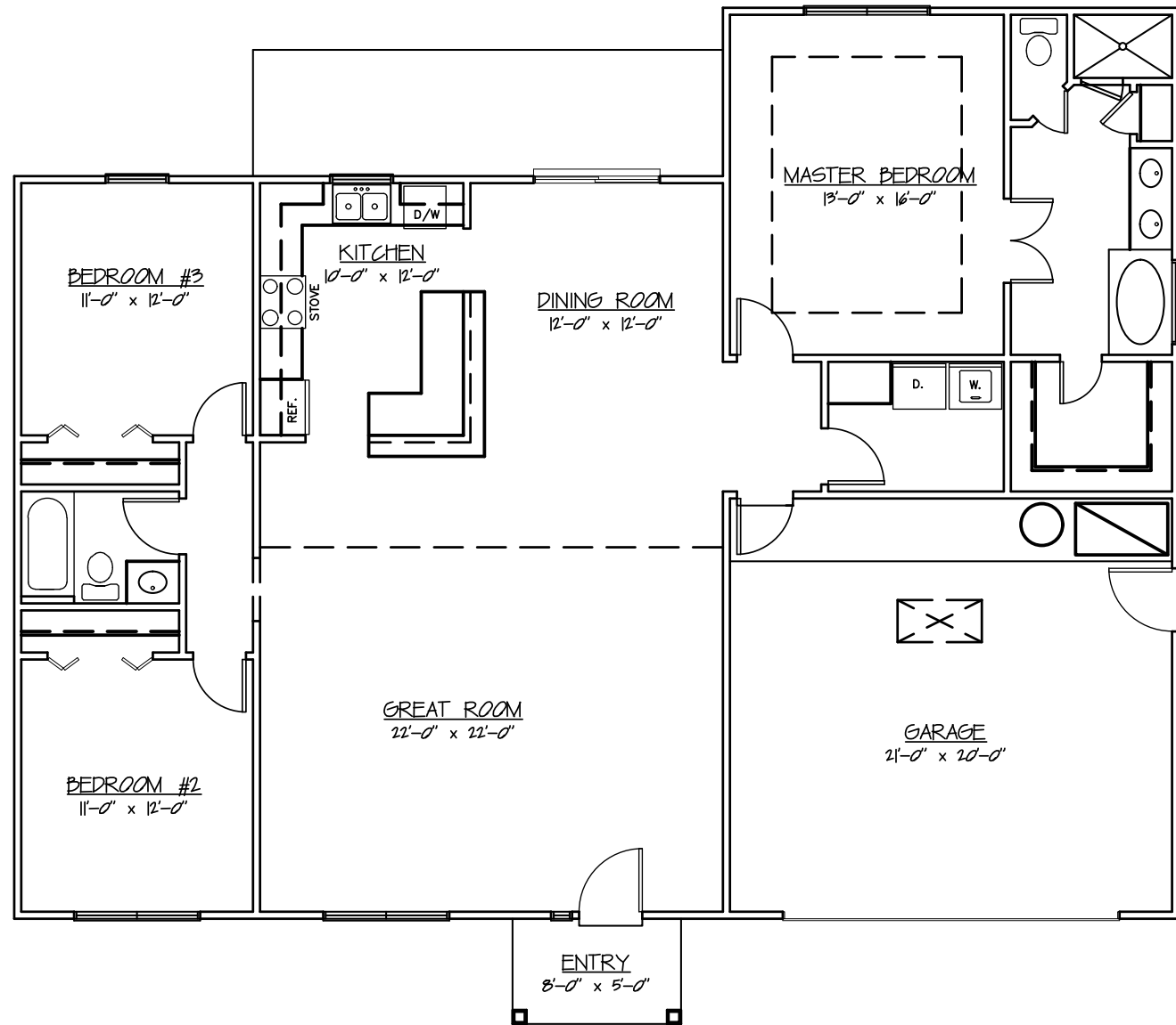
FLOOR PLAN
