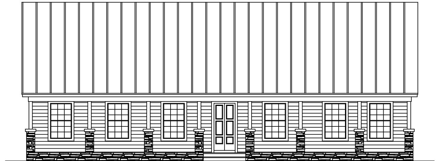
FRONT ELEVATION
