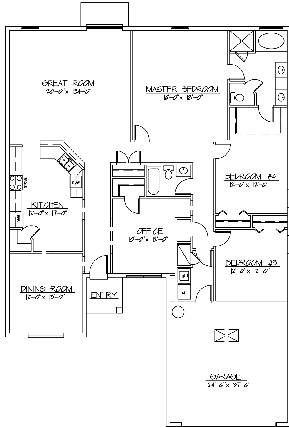
FLOOR PLAN
