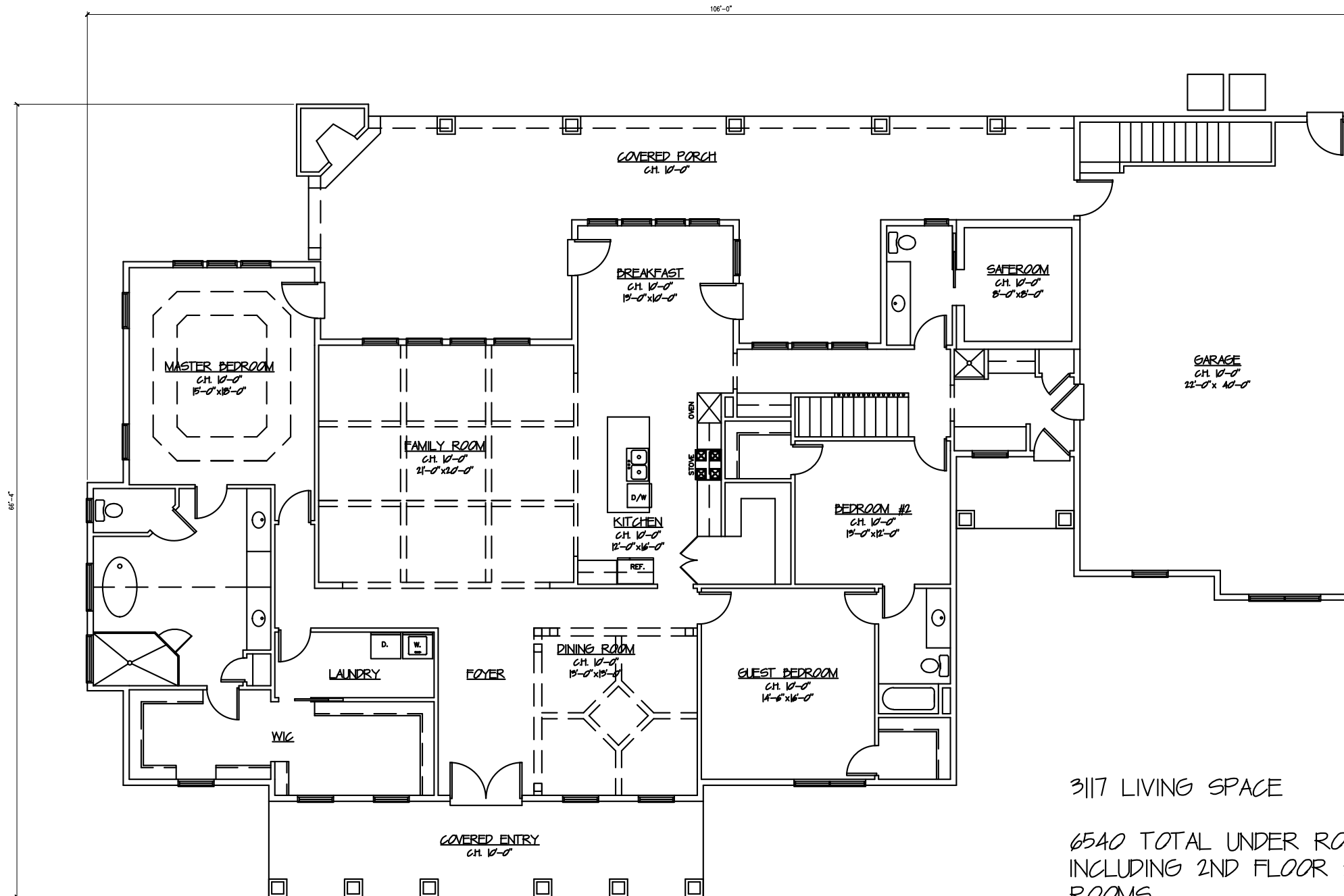
FLOOR PLAN
