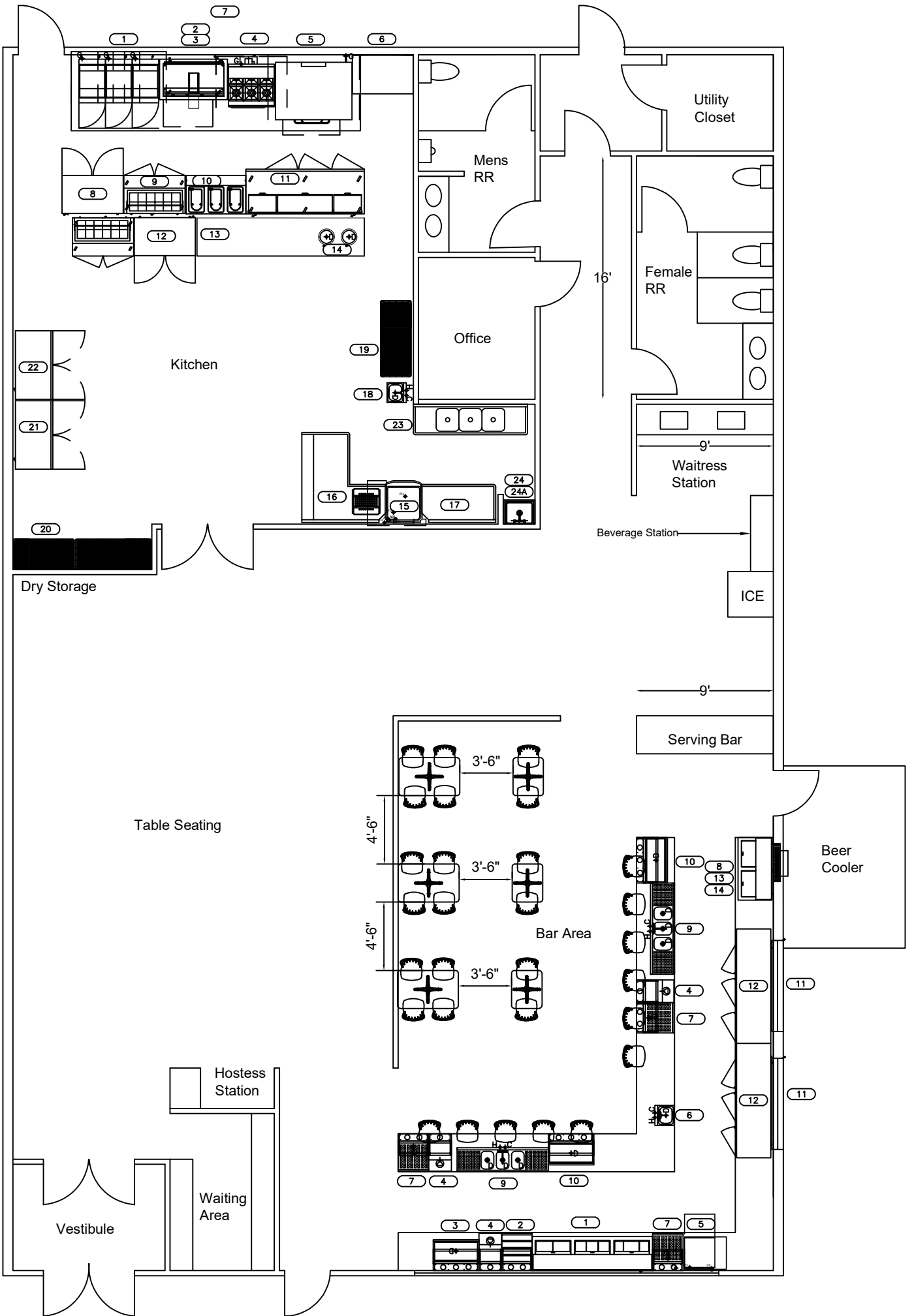
Floor Plan
